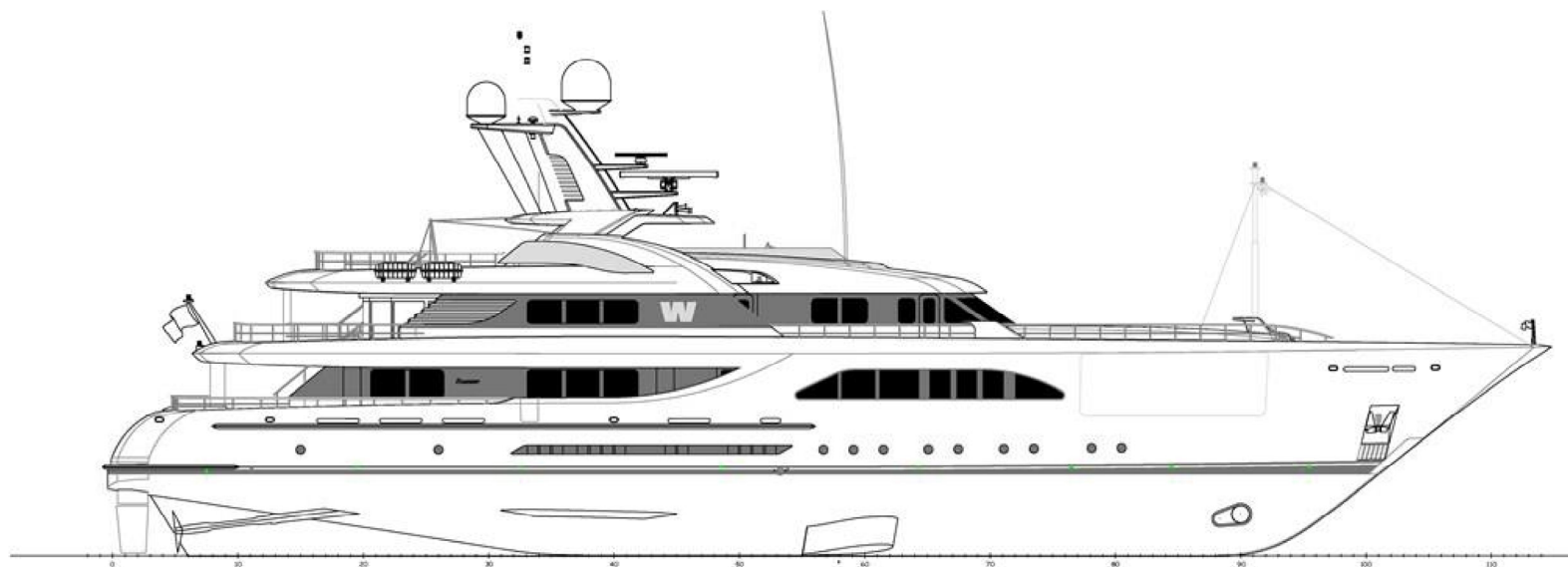
PROFILE
